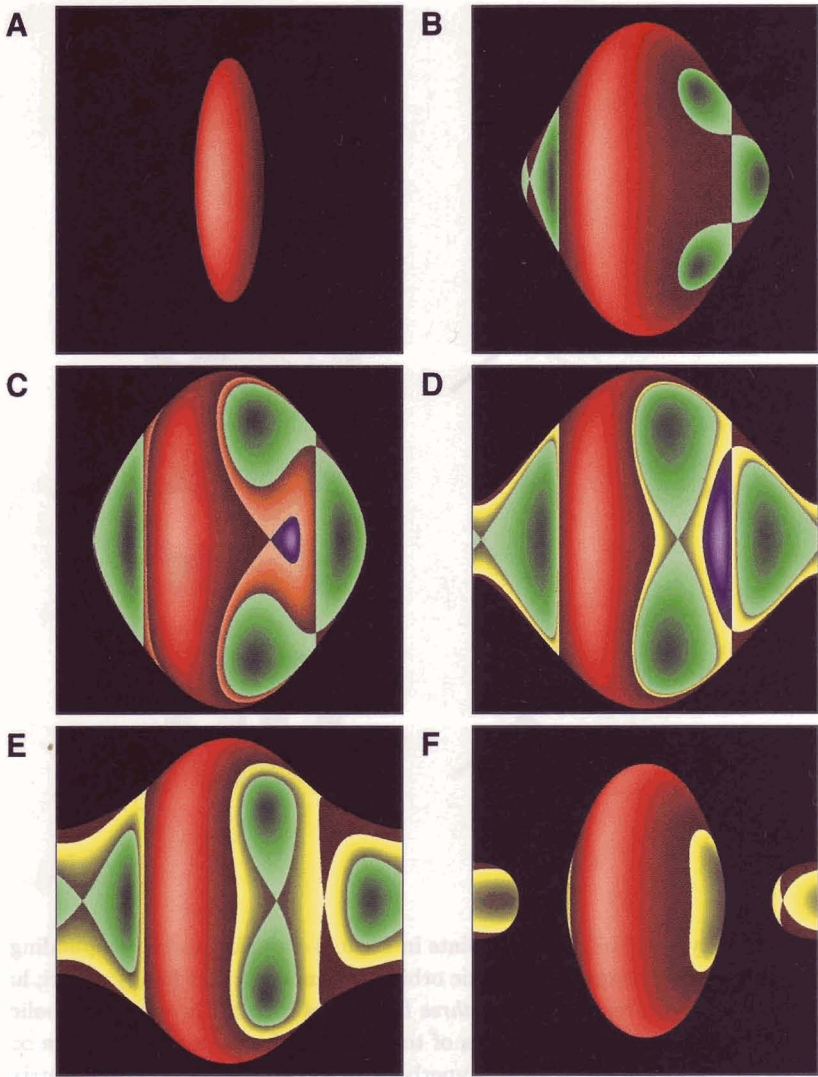
Figure 9. Typical Poincaré surfaces \mathcal{P}_{hl} for the six (h, l) -phases A ... F. From top left to bottom right: A: (-0.5, 1) B: (1.2, 1.58) C: (0.9, 0.34) D: (1.2, 0.4) E: (1.85, 1.43) F: (2.5, 5.3)
