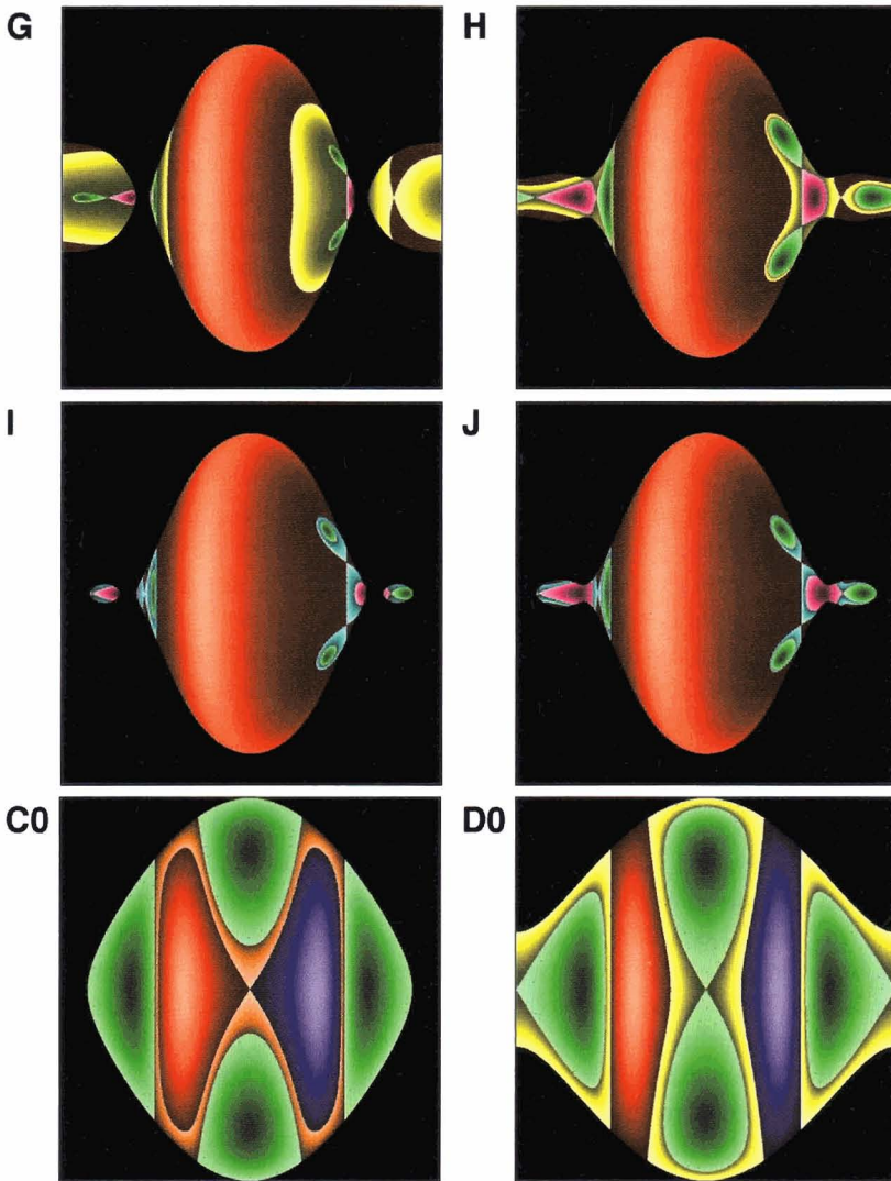
Figure 9. (cont.) \mathcal{P}_{hl} for the (h, l) -phases G ... J and, in the bottom line, C and D with l = 0 . From top left to bottom right: G: (2.5, 4.82) H: (1.85, 3.29) I: (1.8, 3.26) J: (1.8, 3.23) C: (0.9, 0) D:(1.2, 0).
