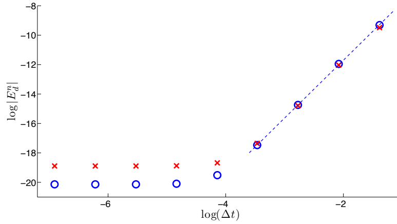
Figure 3: Plot of \log|E_d^n| versus \log(\Delta t) for fixed time of integration T=1 of the system (6.1)-(6.2). The crosses represent results from the PI1 scheme and the circles represent results from the PI2 scheme. The dashed line is a linear regression line with a slope of 3.93.
