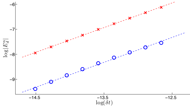
Figure 4: Plot of \log|E_d^n| versus \log(\delta t) for fixed time of integration T=0.18 of the system (6.1)-(6.2). The crosses represent results from the PI1 scheme and the circles represent results from the PI2 scheme. The dashed lines are linear regression lines with a slopes of 0.99 and 1.0, respectively.
