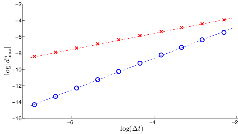
Figure 6: Plot of \log|d_{\max}^n| versus \log(\Delta t) for fixed time of integration T = 1 of the system (6.1)-(6.2). The crosses represent results from the PI1 scheme and the circles represent results from the PI2 scheme. The dashed lines are linear regression lines with slopes of 0.98 and 1.94, respectively.
