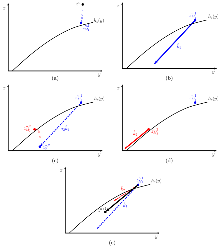
Figure 1: Sketch of the PI1 scheme for a second order Runge-Kutta macrosolver. The microsolver is employed in 1a, 1c, the increments \hat{k}_j are given by vectorfield evaluations in 1b, 1d, and the macrosolver is illustrated in 1e. For this scheme a_1=0 , a_2=1 and b_1=b_2=1/2 .
