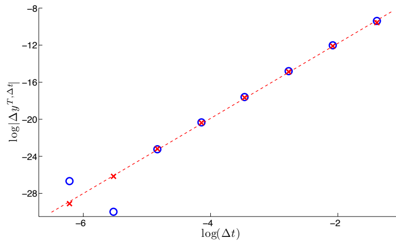
Figure 7: Plot of \log|\Delta y^{T, \Delta t}| versus \log|\Delta t| for fixed time of integration T=1 of the system (6.1)-(6.2). The crosses represent results from the P11 scheme and the circles represent results from the P12 scheme. The dashed line is a linear regression line (of the P11 output) with slope of 4.05.
