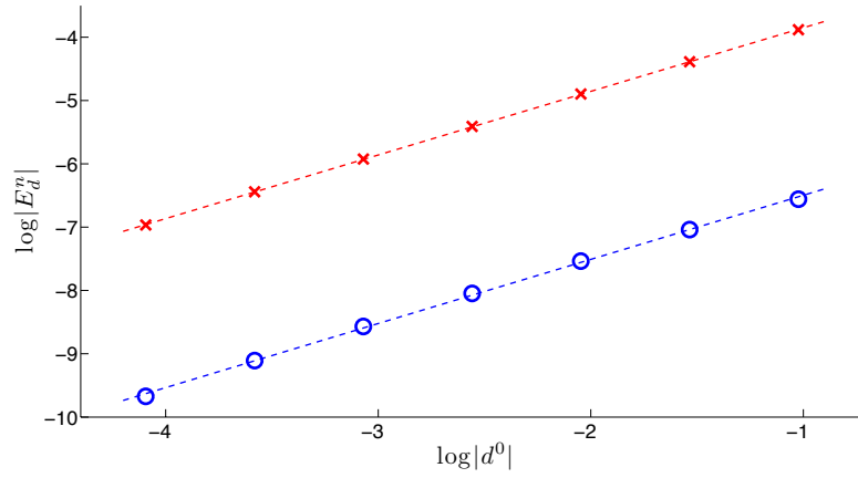
Figure 5: Plot of \log|E_d^n| versus \log|d^0| for fixed time of integration T = 0.0056 of the system (6.1)-(6.2). The crosses represent results from the PI1 scheme and the circles represent results from the PI2 scheme. The dashed lines are linear regression lines with slopes of 1.01.
